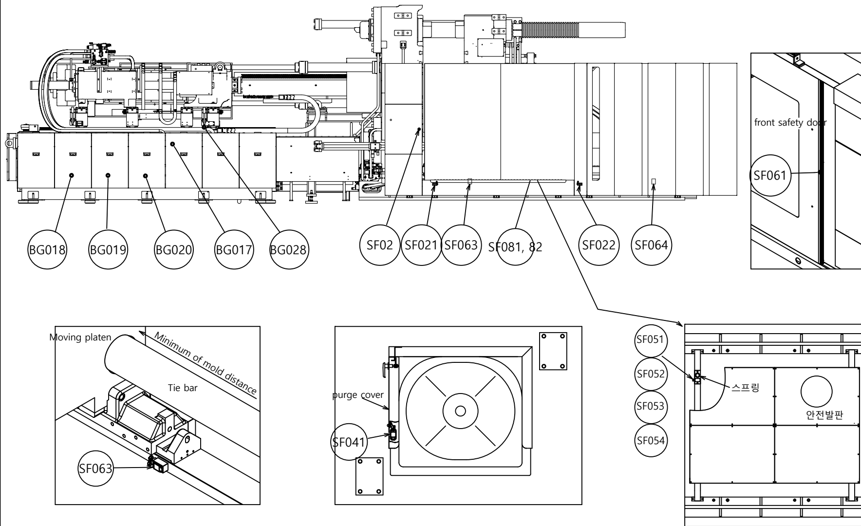
[ The Back of Machine ]
