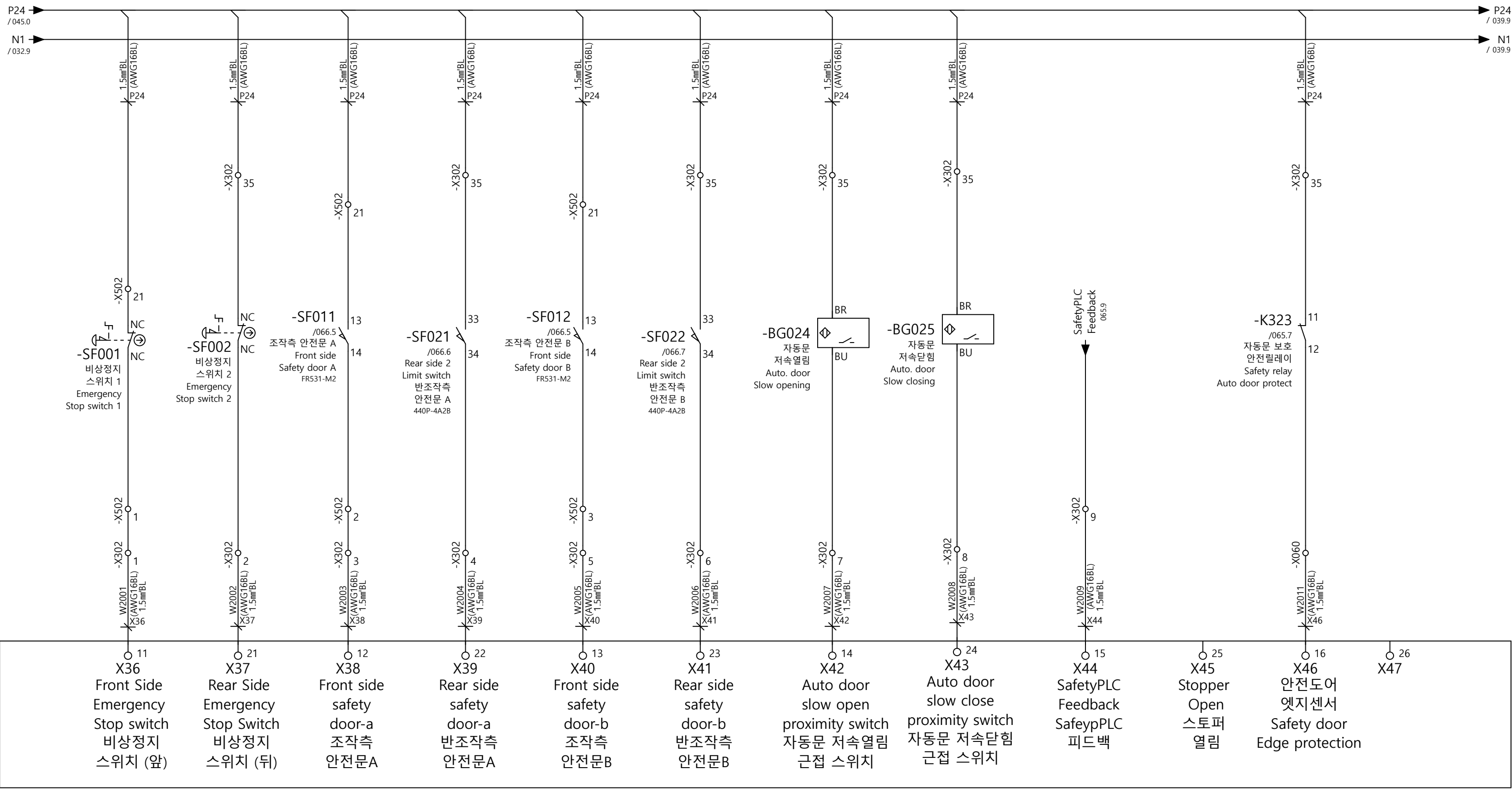
-A308/003.6 DI9371 (Digital input card)
