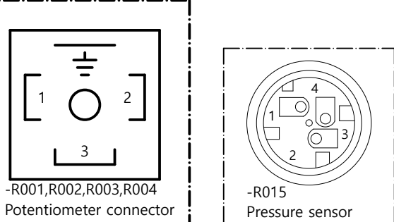
-A304/003.4 AI4632 (Analog Input card)
