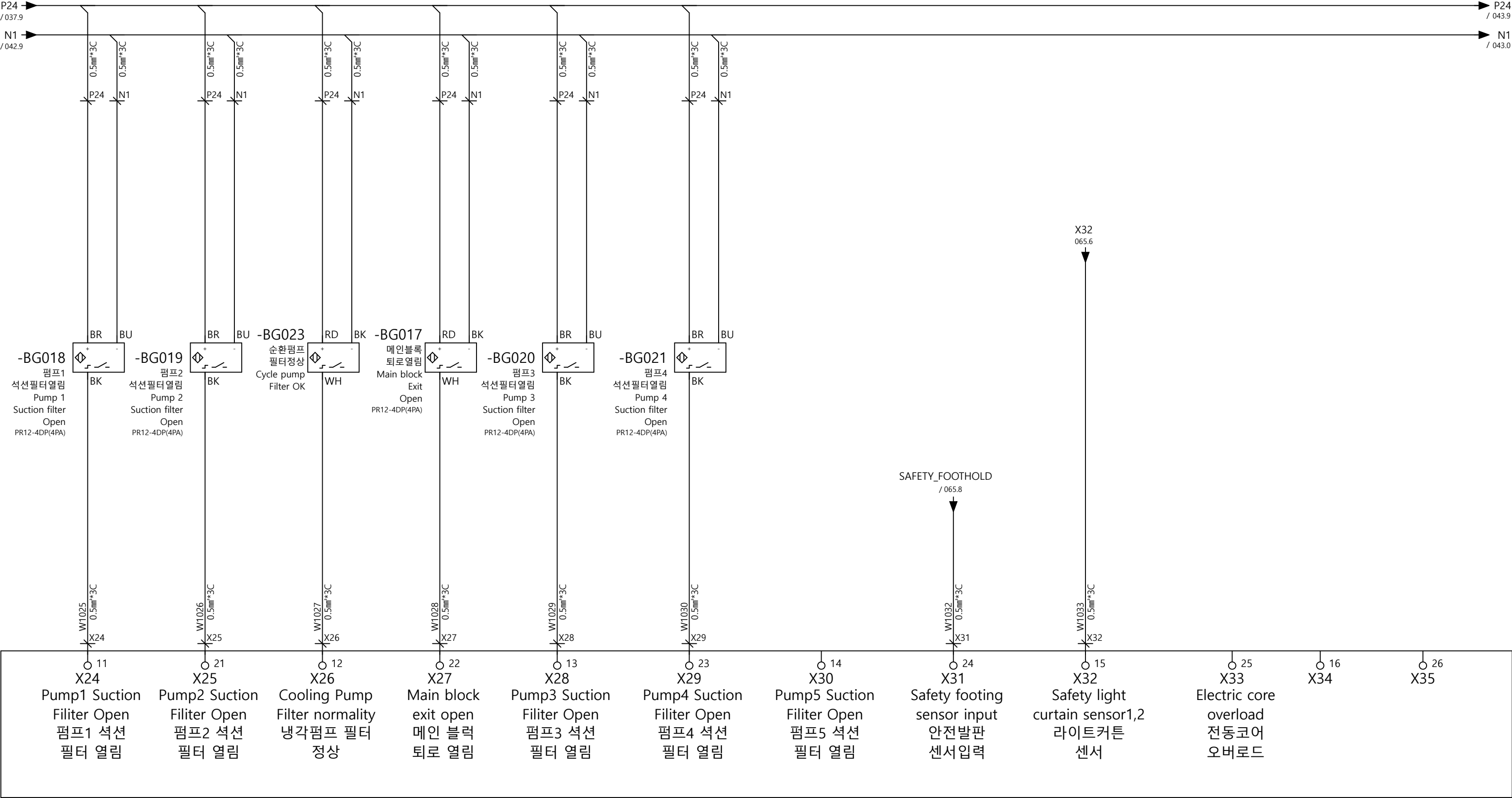
-A209/002.7 DI9371 (Digital input card)
