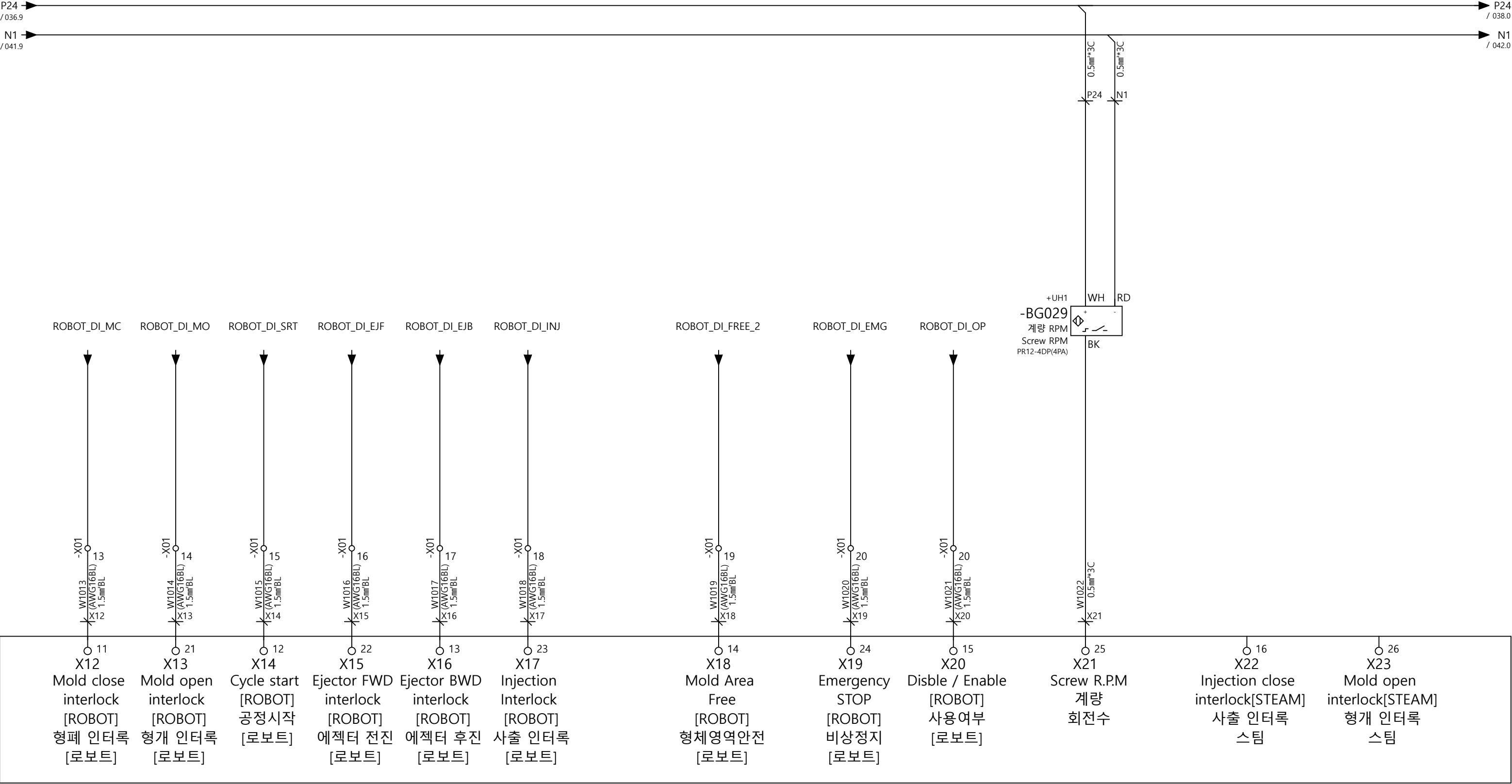
-A208/002.6 DI9371 (Digital input card)
