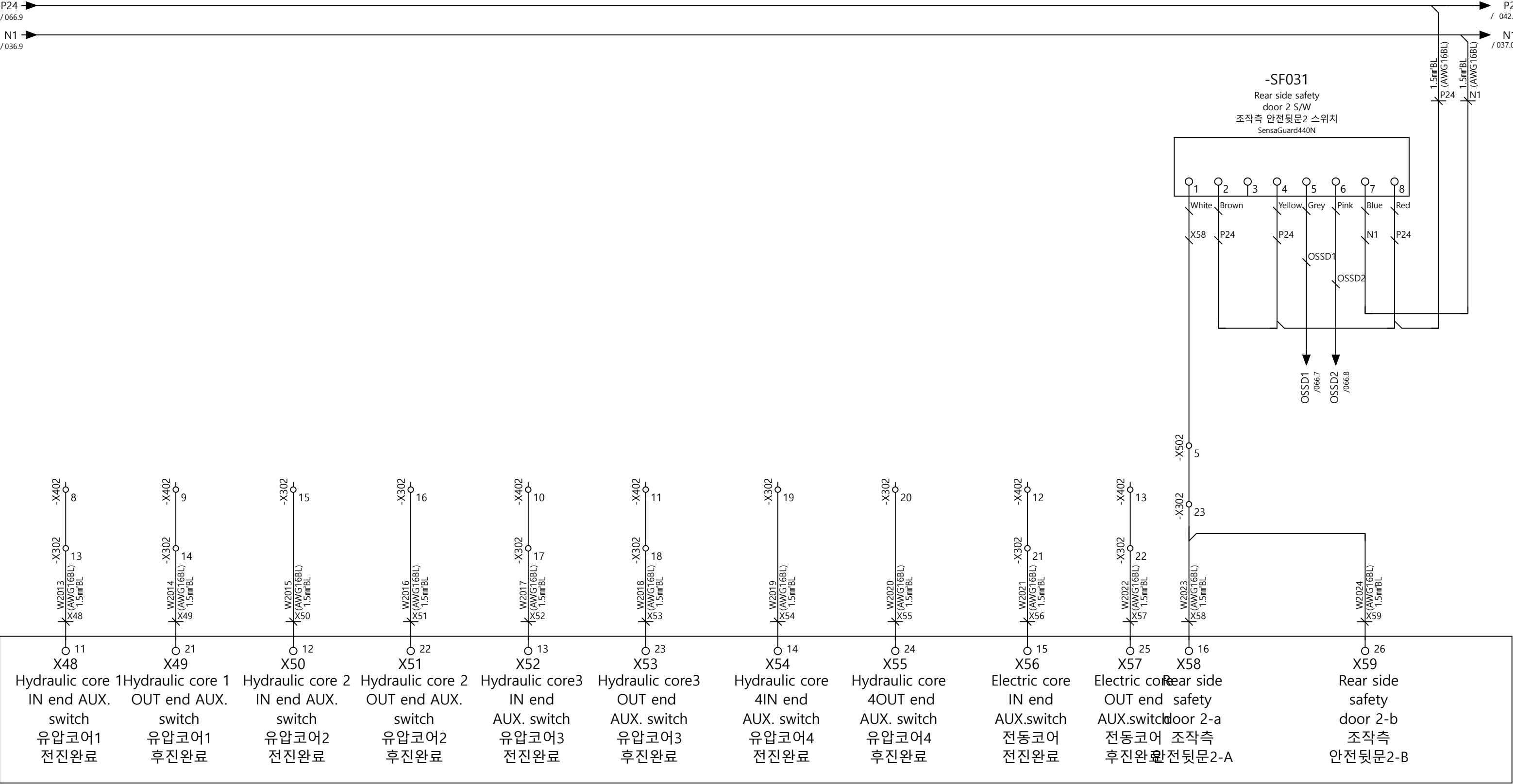
-A309 / 003.6 DI9371 (Digital input card)
